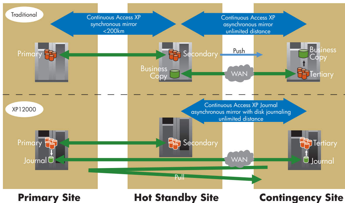
Figure 1. Networks for multisite disaster tolerance
